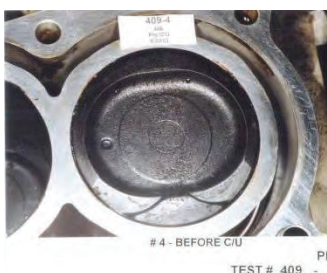
Picture G - Piston before P.i. treatment
