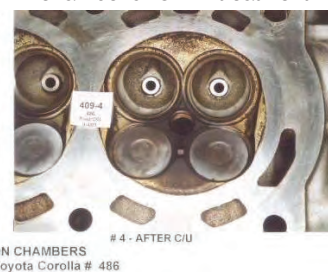
Picture H - Combustion chamber after P.i. treatment
